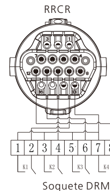
Fig6.20 Conexão inversor – RRCR
